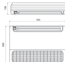
Dimensions: 012-024 models
